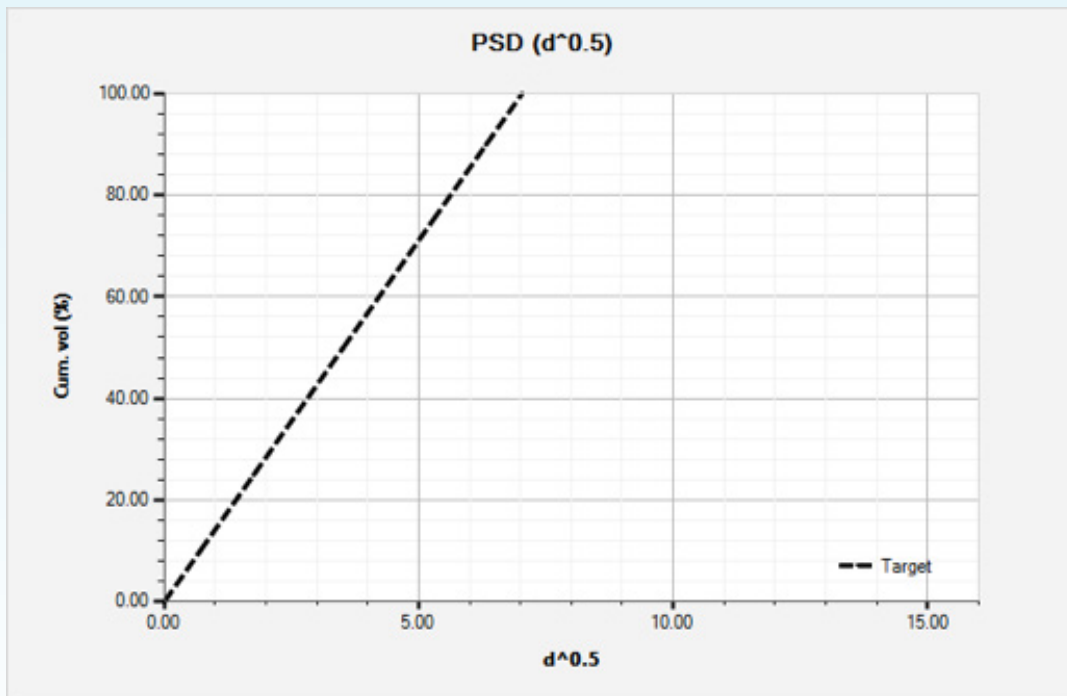
Fig. 2: Ideal packing
