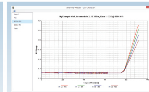
Sensitivity Study - Lost Circulation
