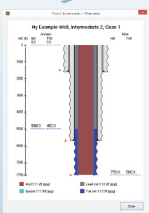
Fluid Schematic
