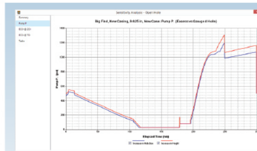
Sensitivity Study - Open Hole Excess
