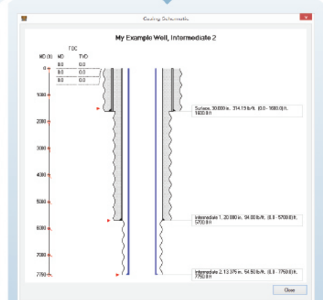
Casing Schematic
