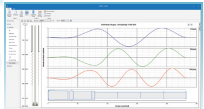
Mode Shape
